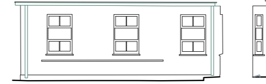
BIG YARD ELEVATION F&G
