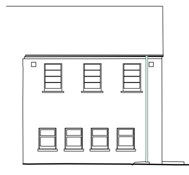
SMALL YARD ELEVATION E
